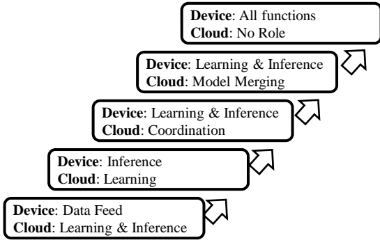
Fig. 1. Evolution of Capabilities in Cognitive Operations Plane
