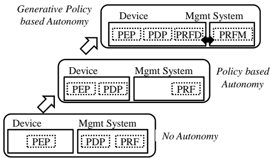
Fig. 4. Evolution of PBMS architectures [11].
