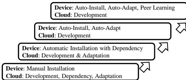
Fig. 2. Evolution of Capabilities in Development Plane
