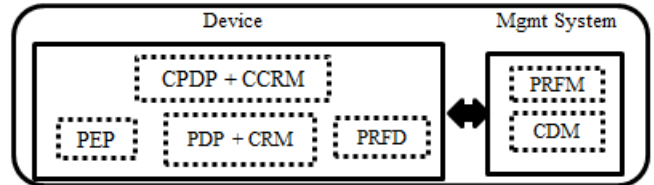
Fig. 5. Decentralized P2P generative policy architecture. Legend: PDP+CRM: PDP enhanced with conflict resolution management (CRM); CPDP+CCRM: Collaborative PDP enhanced with collaborative CRM; CDM: collaborative device management
