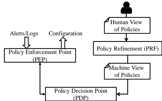
Fig. 3. High Level Reference Architecture for PBMS [12].
