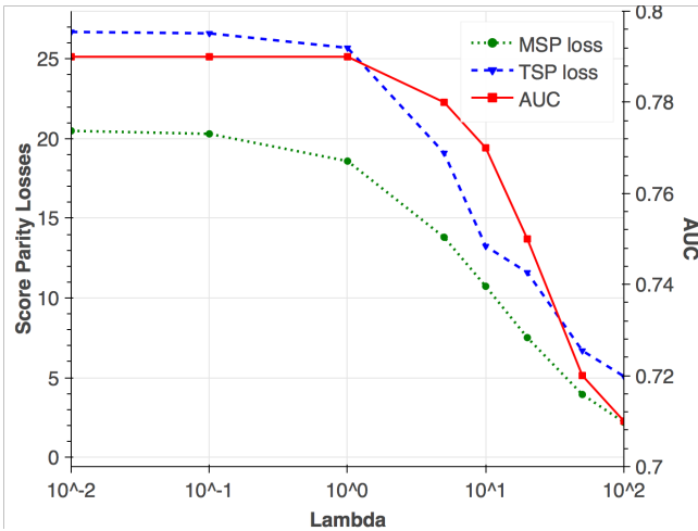
Figure 2: Variation of score parities and AUC with the TFCS trade-off parameter \lambda for the MEPS dataset.
