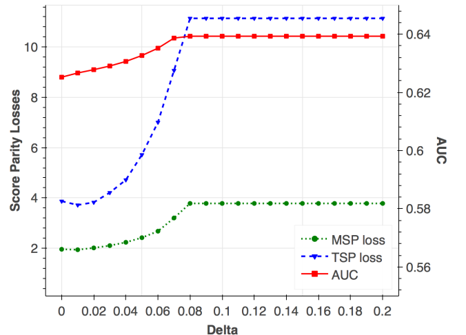
Figure 3: Variation of score parities and AUC with the PCCS trade-off parameter \delta for the Mobile Money dataset.
