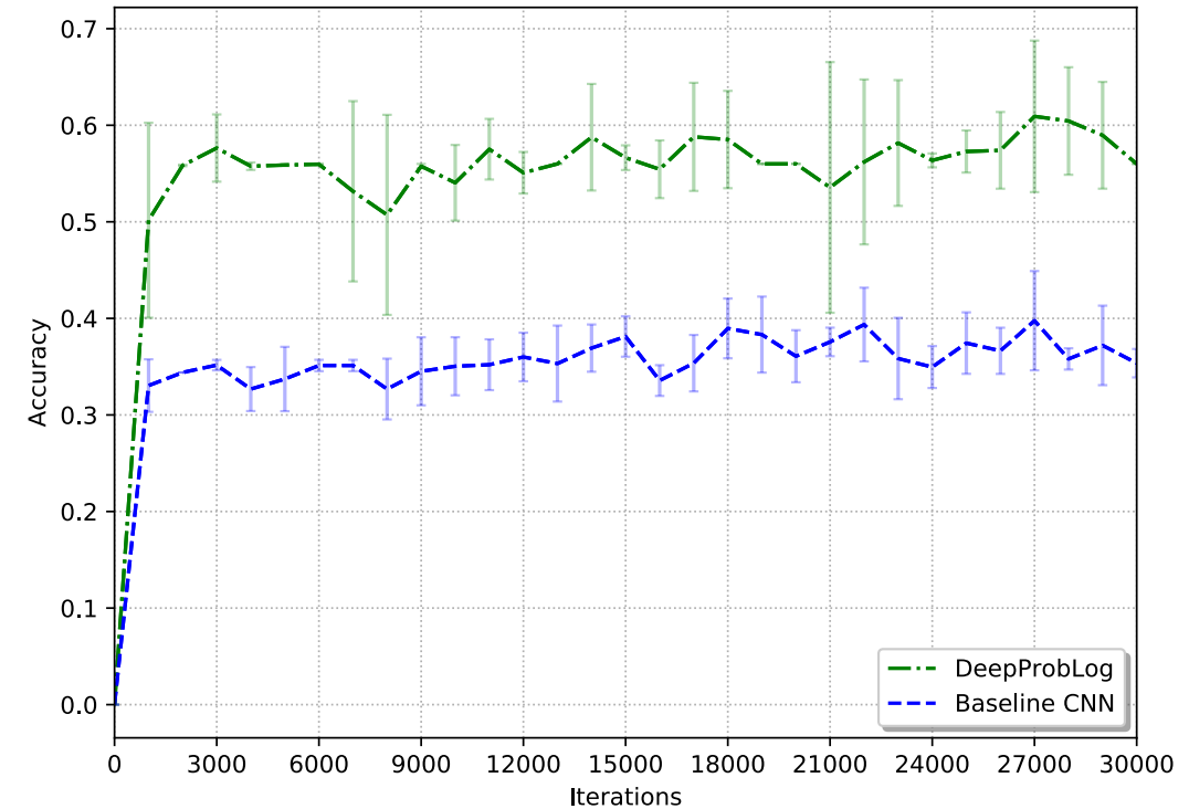
DeepProbLog Accuracy vs Baseline end-end CNN over 5 training runs.
