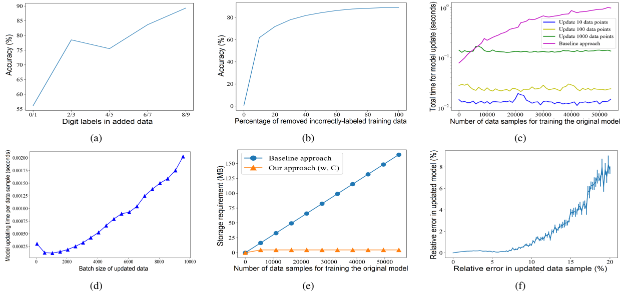
Fig. 1. Experimentation results: (a) model accuracy when incrementally adding each group of data; (b) model accuracy after removing different percentages of incorrectly-labeled training data; (c) total time for model update/retraining; (d) normalized model updating time per data sample (total updating time/batch size) of our proposed method; (e) storage requirement; (f) error of updated model using our proposed method caused by inaccuracies in removed training data samples.
