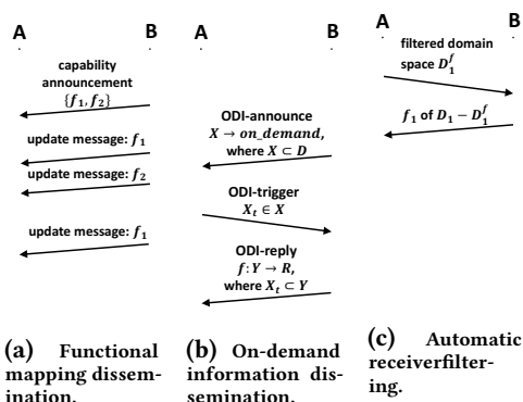
Figure 1: The message-time diagrams of SFP protocol.
